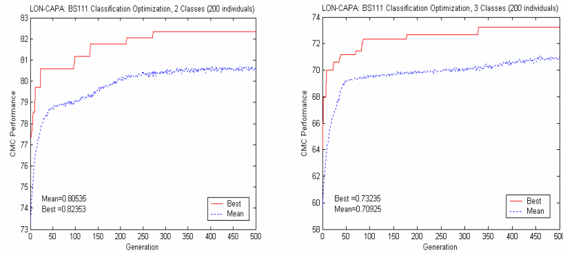
Fig. 2. GA-Optimized Combination of Multiple Classifiers’ (CMC) performance in the case of 2- and 3-Classes, 200 weight vectors individuals, 500 Generations
